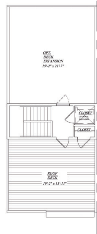
Roof Plan
